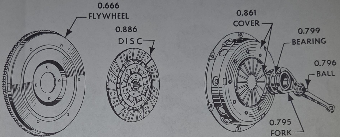
DIAPHRAGM CLUTCH—RIVETTED TYPE
