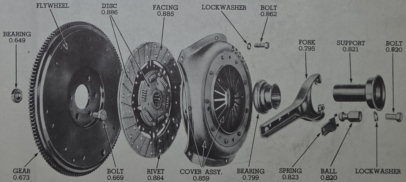
CLUTCH AND FLYWHEEL
