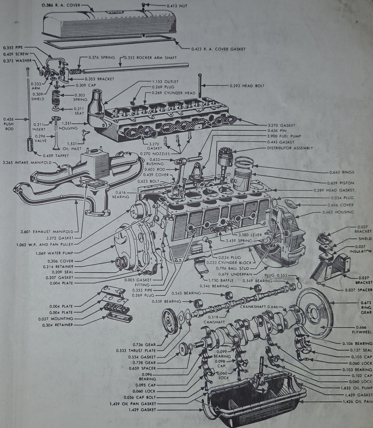
"261" ENGINE — EXPLODED VIEW
