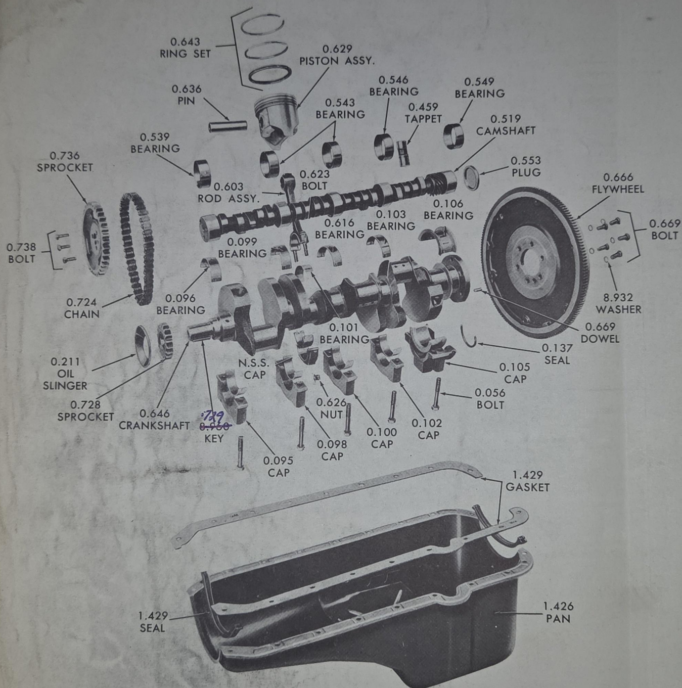
V-8 ENGINE - EXPLODED 20-22
