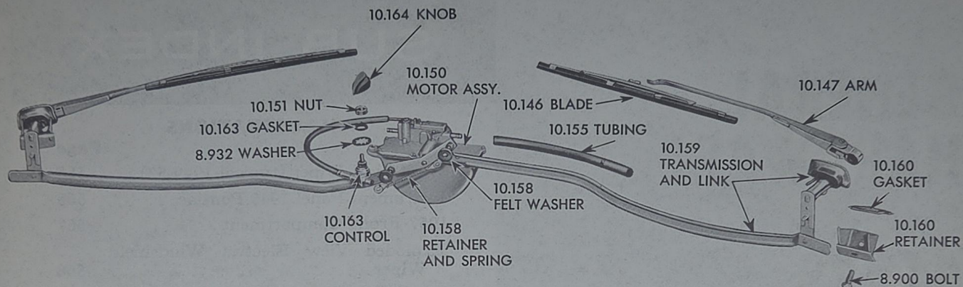
1949 THROUGH 51 WINDSHIELD WIPER
