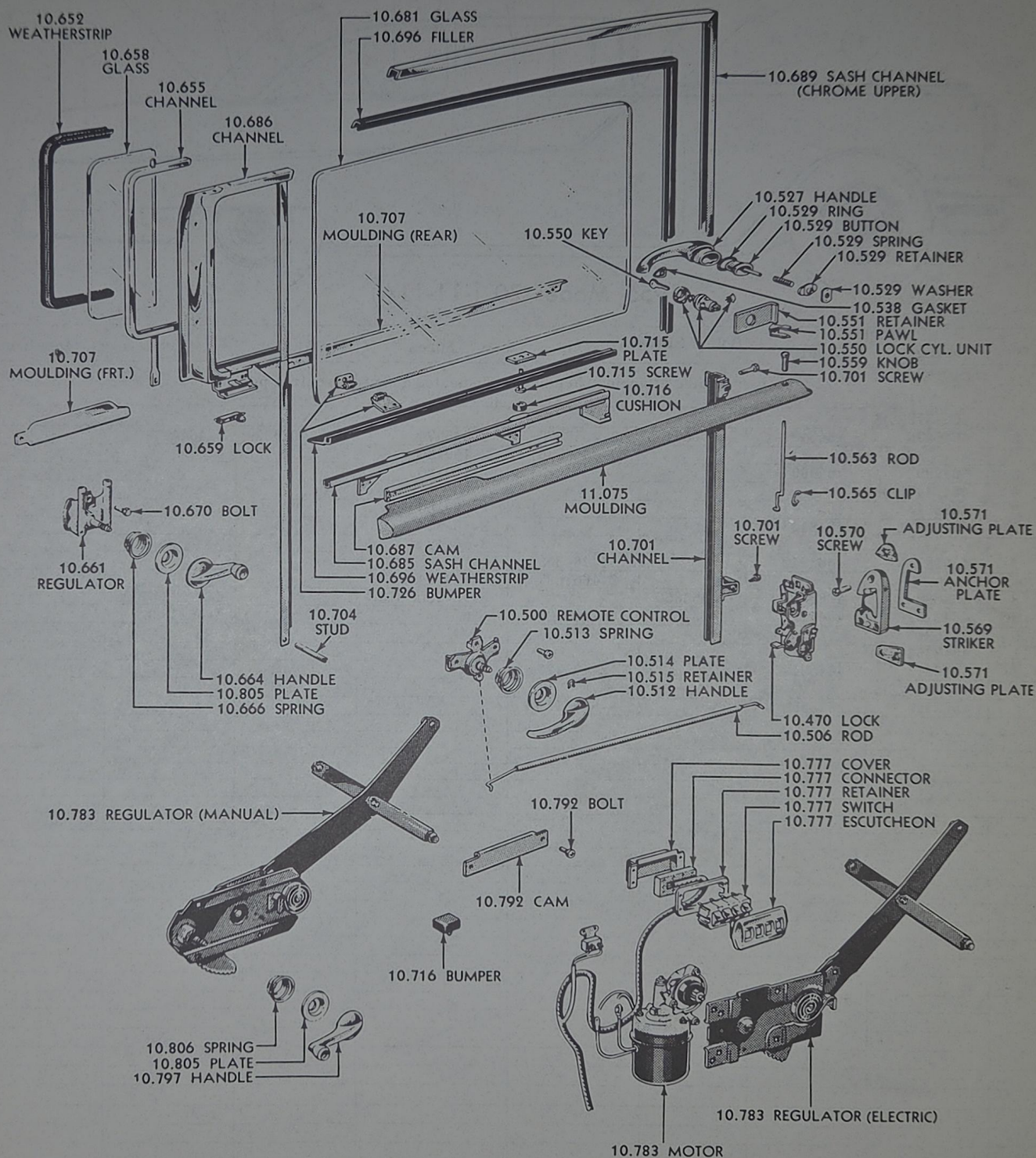
FRONT DOOR HARDWARE LAYOUT
