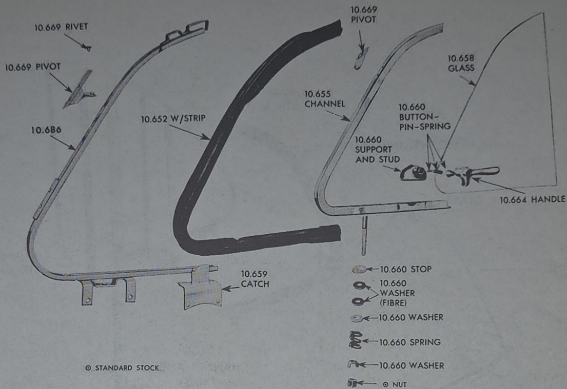
FRONT DOOR VENTILATOR (Less Division Channel)
