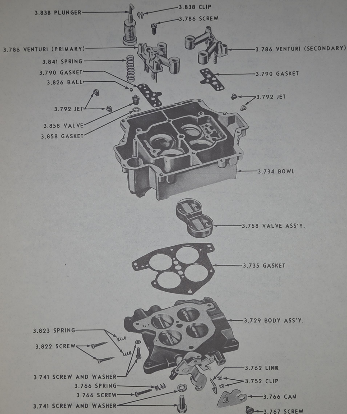
Rochester Carburetor Float Bowl and Throttle Body 1956 4BC
