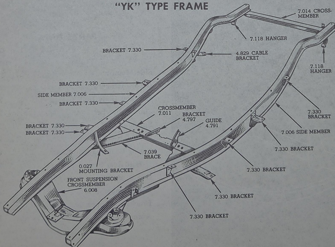
FRAME TYPES
