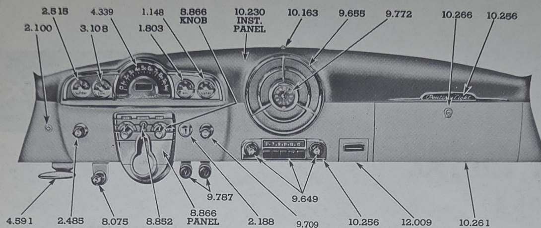
1949 INSTRUMENT PANEL
