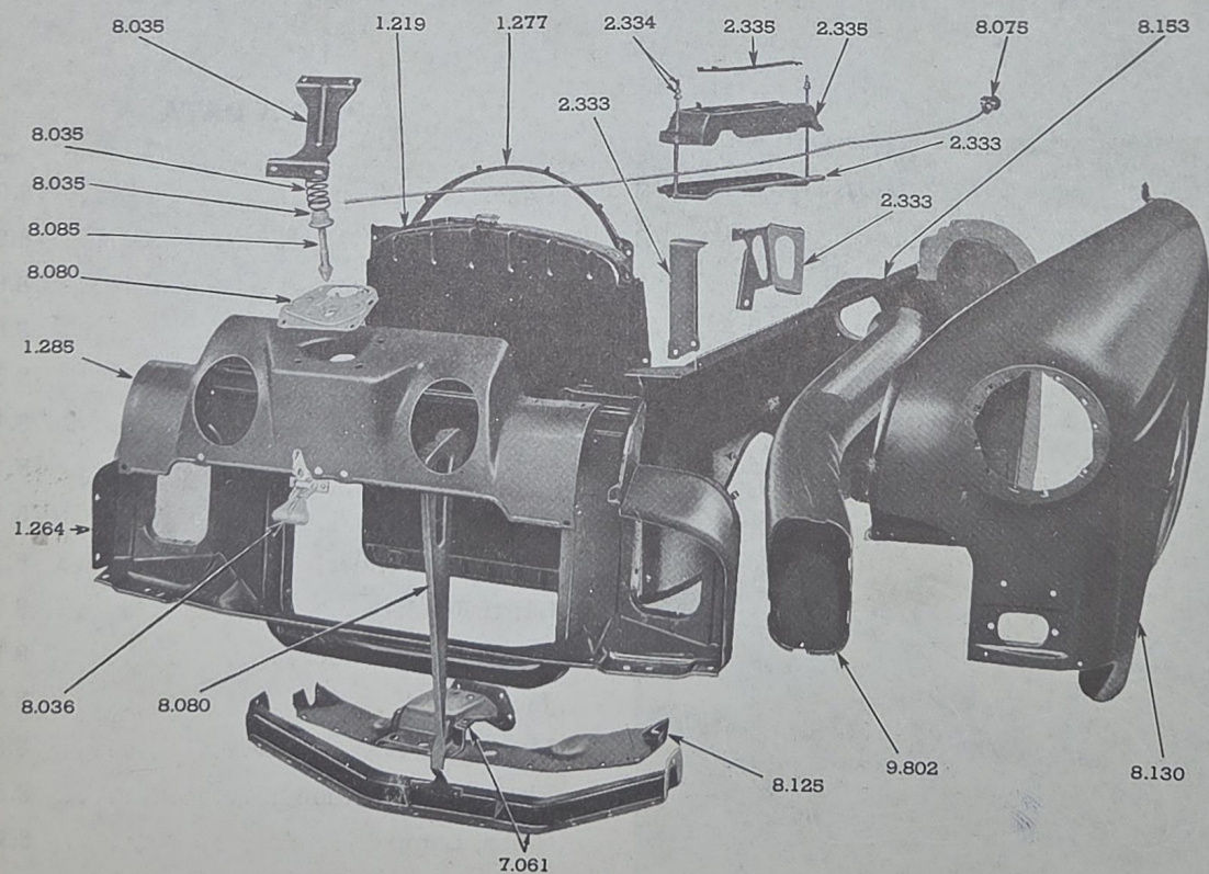
1950 SHEET METAL
